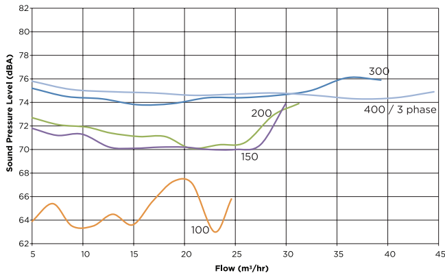
Noise Level
