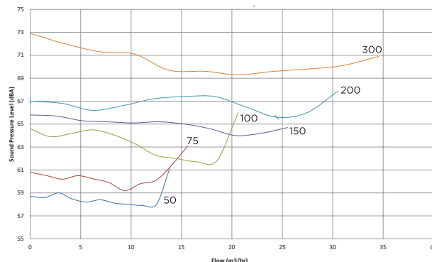
Noise Curve
