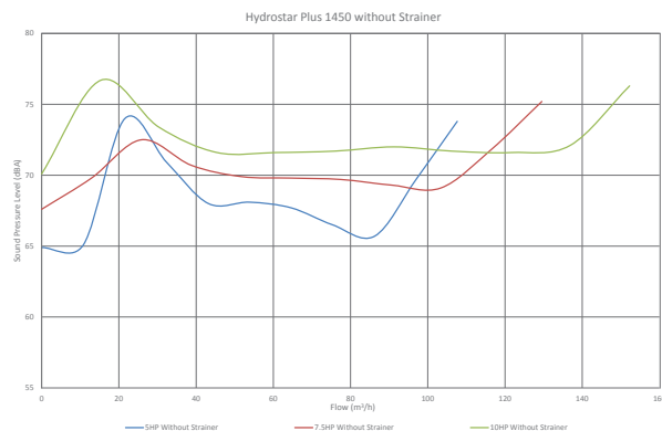
Noise Curve
