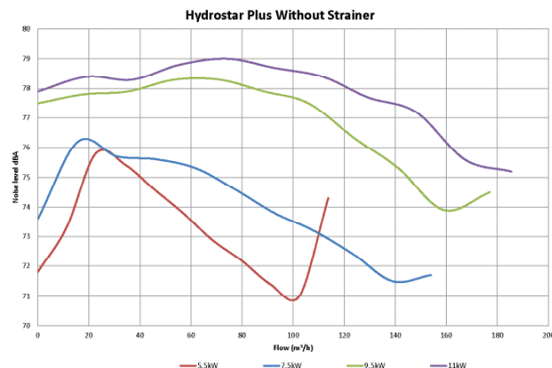
Noise Curve
