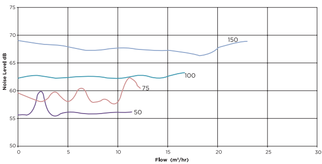
Noise Curve
